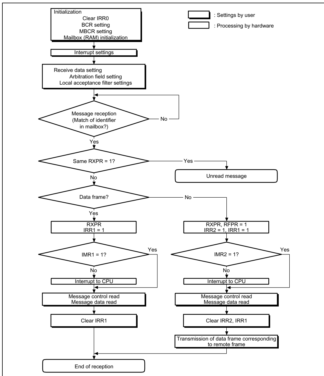
Figure 15-11 Reception Flowchart
