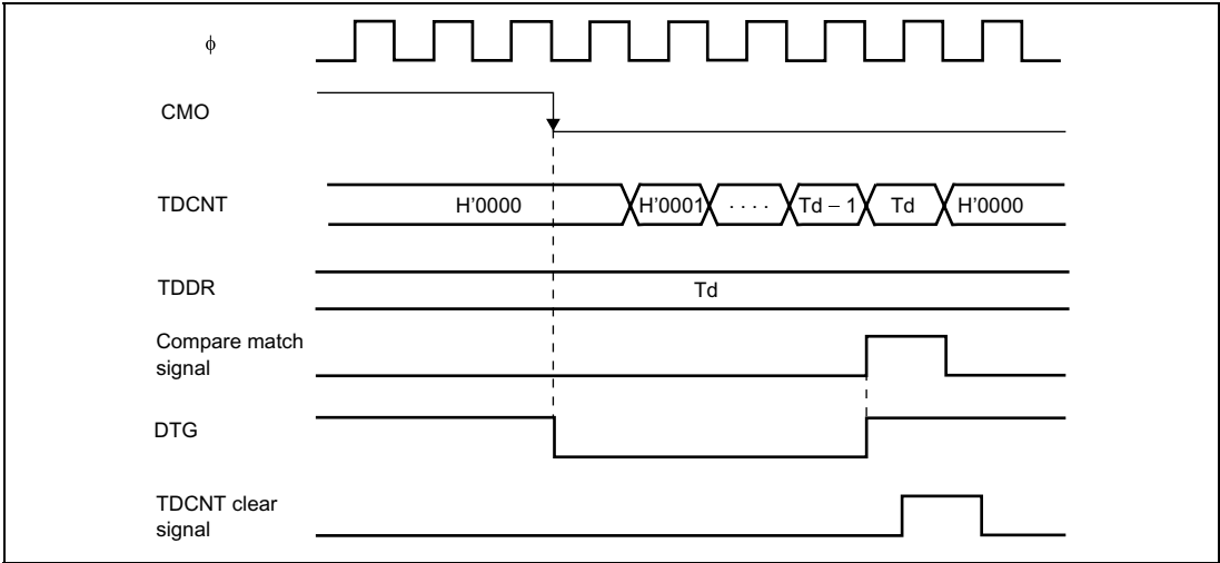
Figure 11-11 TDCNT Operation Timing
