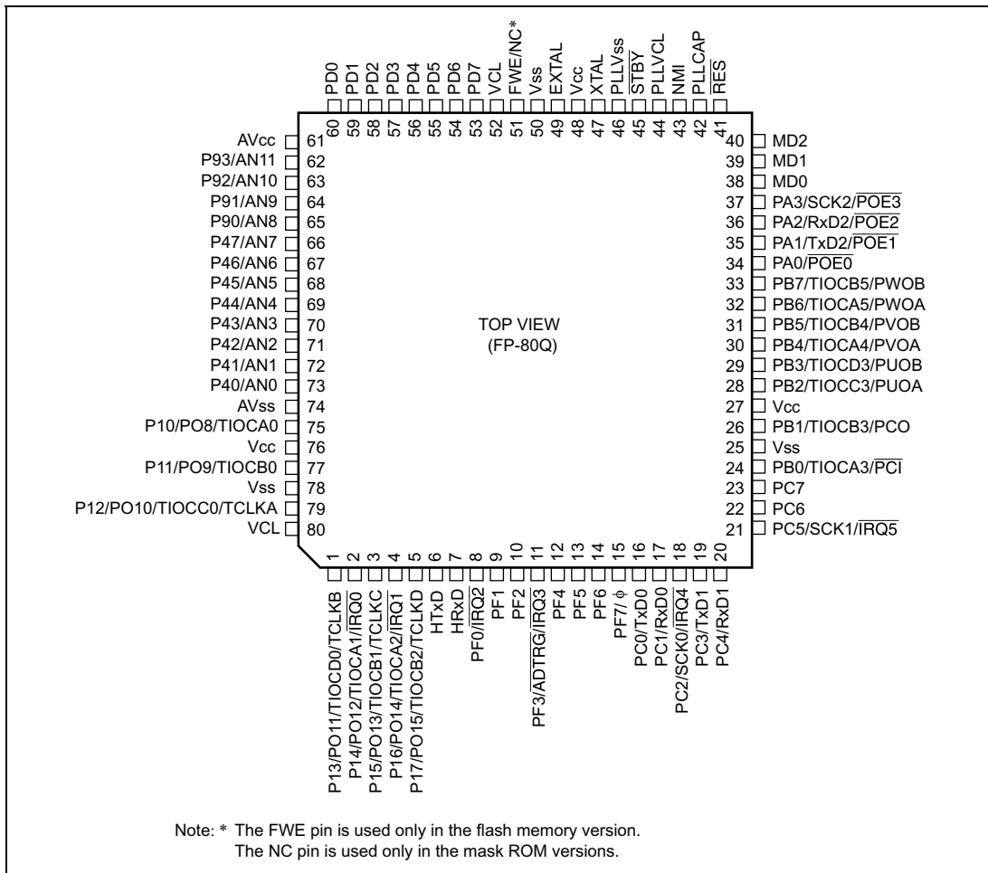
Figure 1-2 Pin Arrangement
