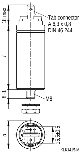
Dimensional drawing 3 Tab connectors 6,3 mm
