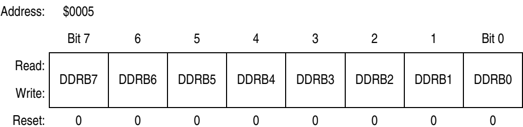
Figure 22-6. Data Direction Register B (DDRB)
