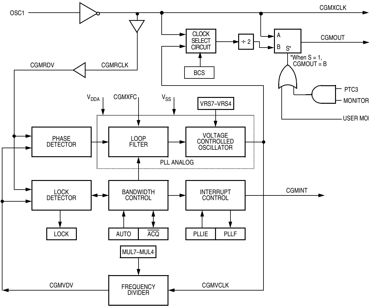
Figure 10-1. CGM Block Diagram
