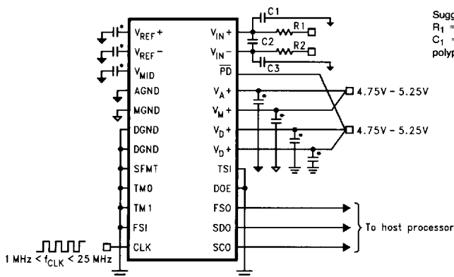
FIGURE 9. Typical Connection Diagram for the ADC16471
