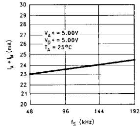
Analog Supply Current ( I_A + I_M ) vs Output Data Rate
