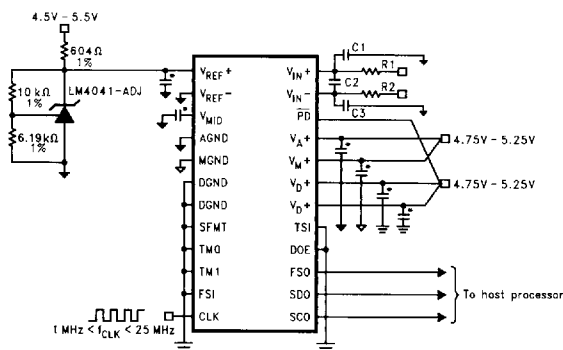
FIGURE 10. Typical Connection Diagram for the ADC16071
