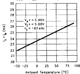
Analog Supply Current ( I_A + I_M ) vs Temperature
