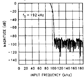
Frequency Response of Digital Filter
