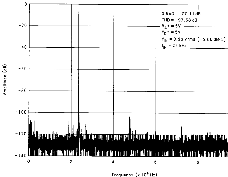
FIGURE 6. Typical Performance of the ADC16071/ADC16471 at f_S = 192 \text{ kHz} , f_{IN} = 24 \text{ kHz}
