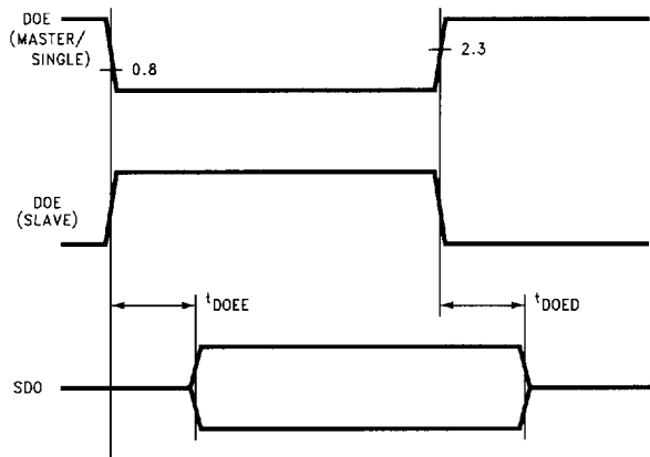
FIGURE 5. Timing Diagrams for Data Output Enable (DOE) and Serial Data Out (SDO)
