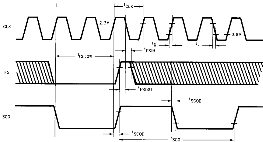
FIGURE 1. Timing Diagrams for Clock Input (CLK), Frame Sync Input (FSI), and Serial Clock Output (SCO)
