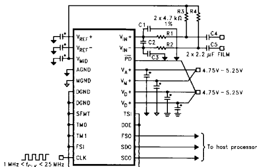
FIGURE 10. Typical Connection Diagram for the ADC16071
