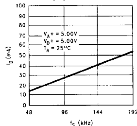
Digital Supply Current ( I_D ) vs Output Data Rate
