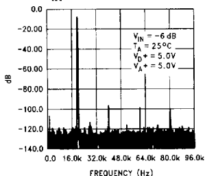
Spectral Response, f_S = 192 kHz, f_{IN} = 20 kHz
