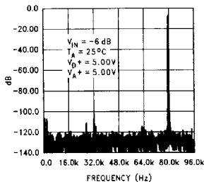
Spectral Response, f_S = 192 kHz, f_{IN} = 80 kHz
