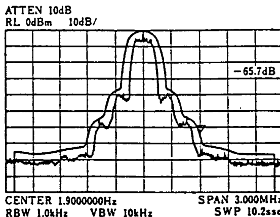
Output Spectrum
