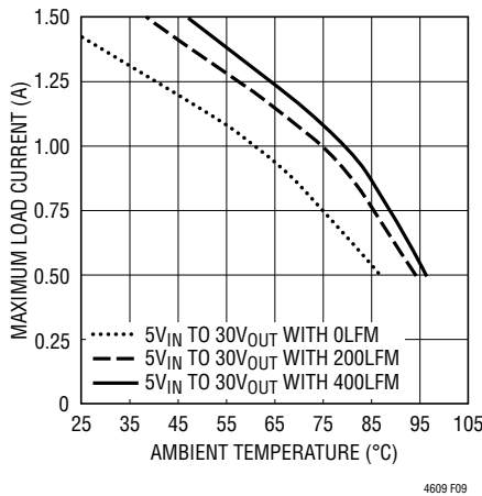
Figure 9. 5V IN to 30V OUT without Heat Sink
