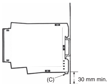
Rail stopper
