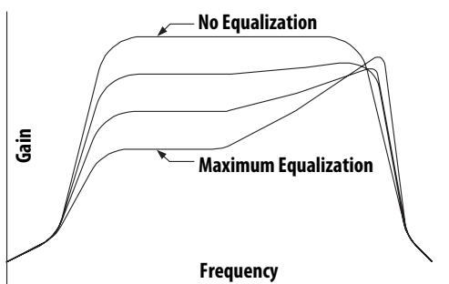
Figure 4. Input Equalization
