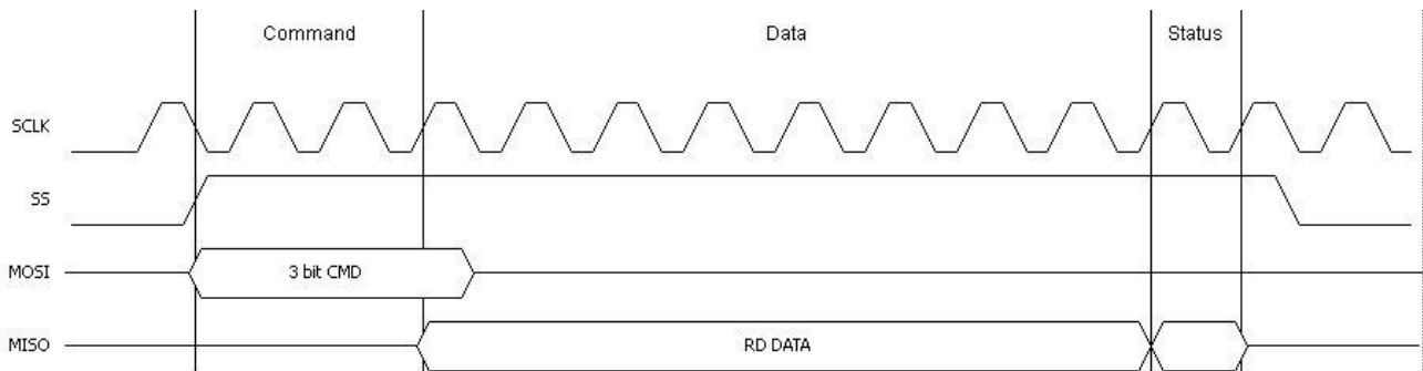
Figure 6.14 VNC1L Mode Data Read
