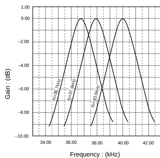
Fig.6 BPF characteristic
