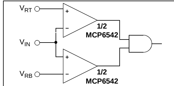
FIGURE 4-12: Windowed Comparator.
