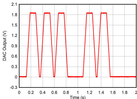
Figure 73. High-Priority Alarm
