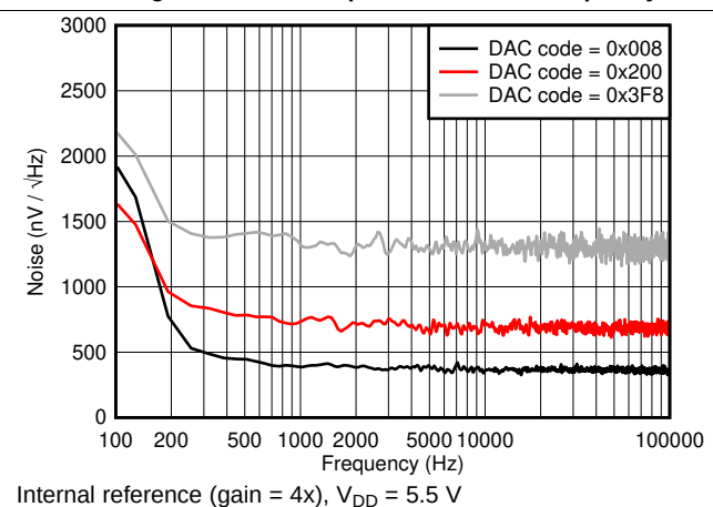
Figure 45. DAC Output Noise Spectral Density
