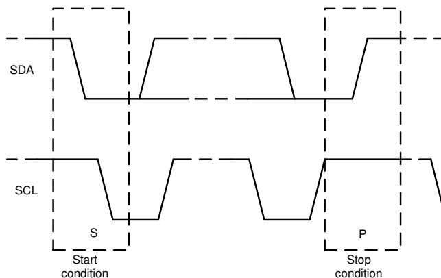
Figure 51. Start and Stop Conditions
