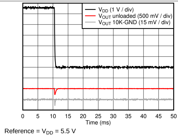
Figure 41. Power-off Glitch
