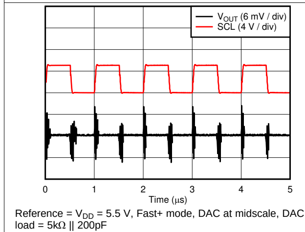
Figure 42. Clock Feedthrough
