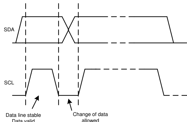
Figure 52. Bit Transfer on the I 2 C Bus
