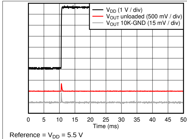
Figure 40. Power-on Glitch
