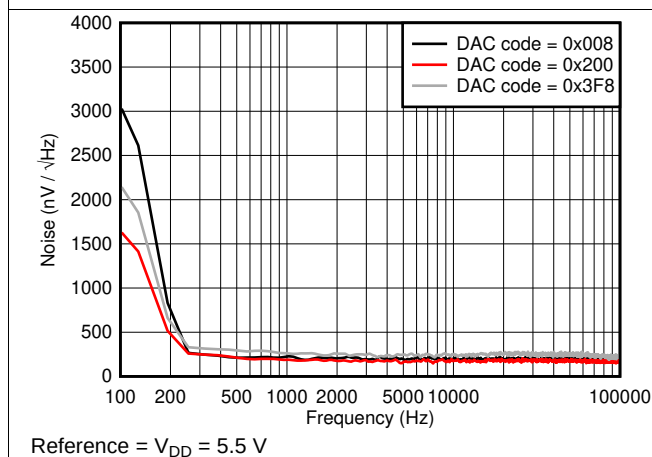
Figure 44. DAC Output Noise Spectral Density
