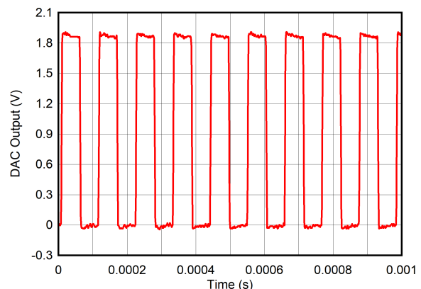
Figure 74. Pulse Frequency
