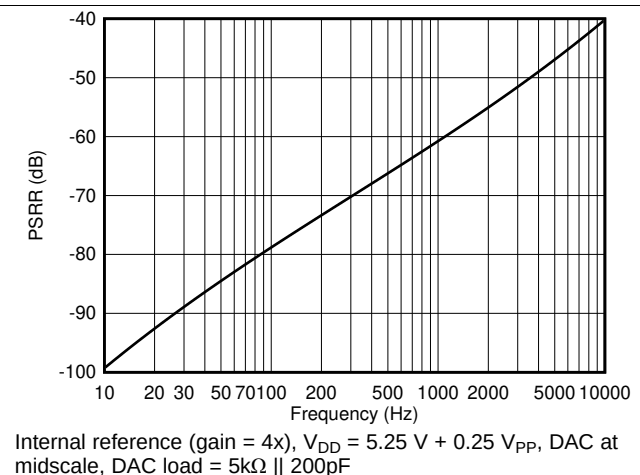
Figure 43. DAC Output AC PSRR vs Frequency
