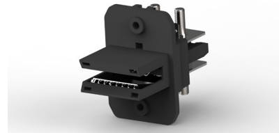
Dual Pole 500A Connector 2204866-1
