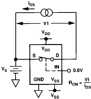
TEST CIRCUIT 1
