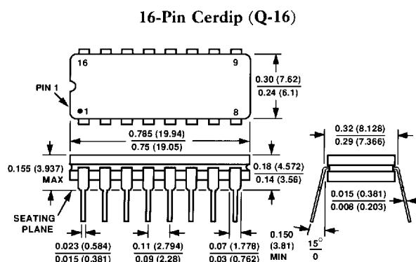
LEAD NO. 1 IDENTIFIED BY DOT OR NOTCH LEADS ARE SOLDER OR TIN-PLATED KOVAR OR ALLOY 42
