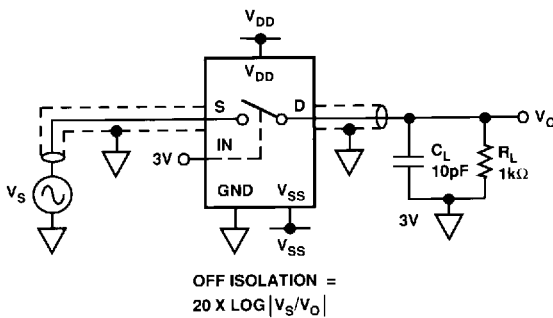
TEST CIRCUIT 5
