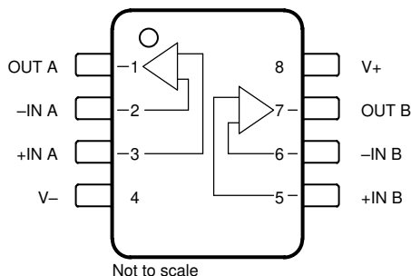
Figure 4-2. OPA2131 D Package, 8-Pin SOIC (Top View)
