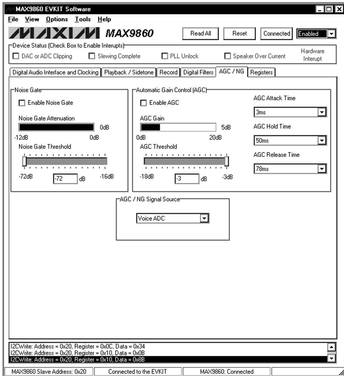
Figure 6. MAX9860 Evaluation Software (AGC / NG Tab)
