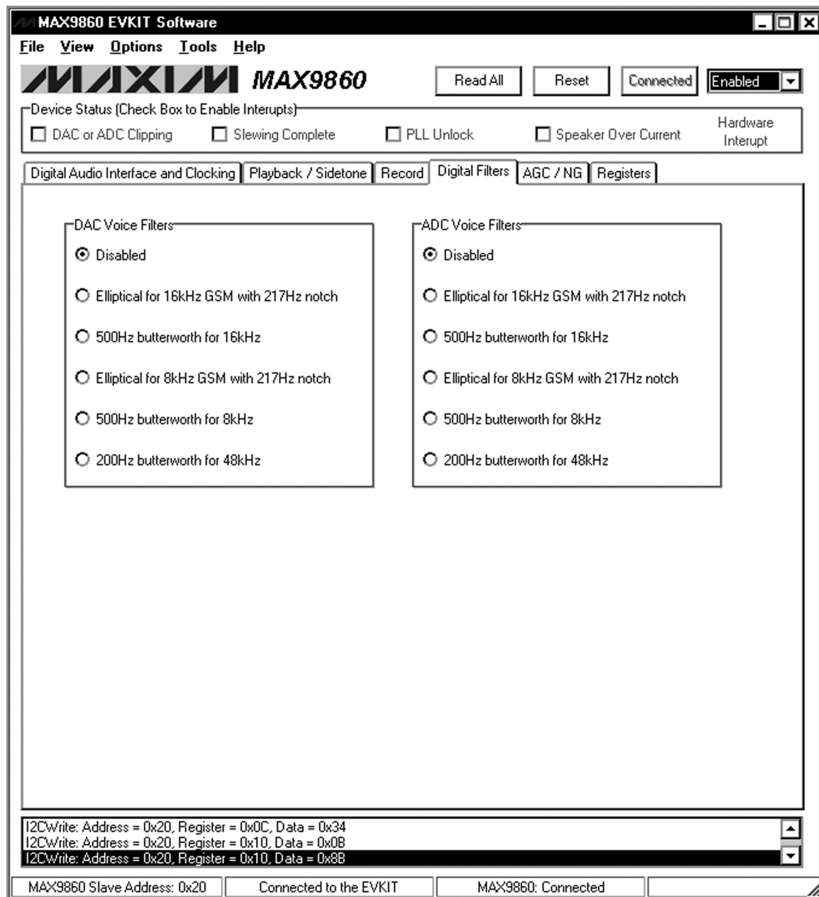
Figure 5. MAX9860 Evaluation Software (Digital Filters Tab)
