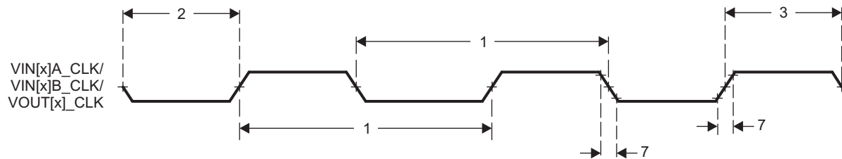
Figure 8-38. HDVPSS Clock Timing
