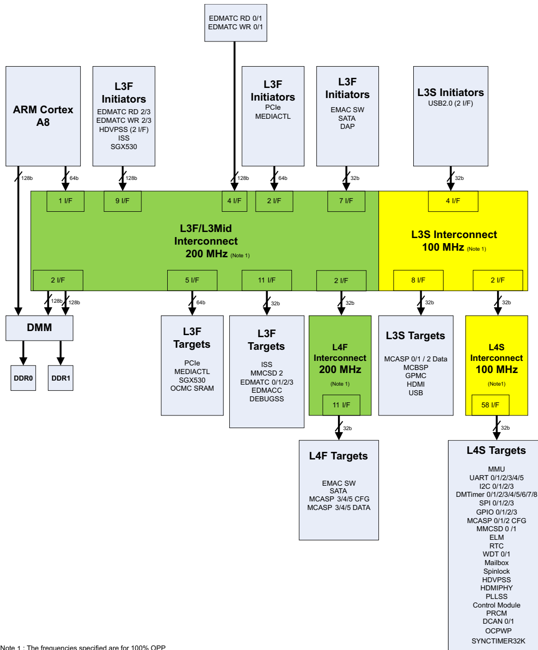
Figure 5-1. System Interconnect
