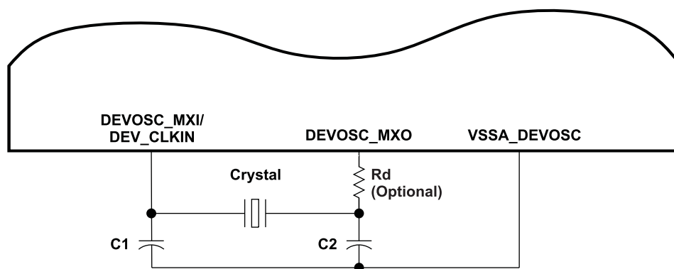
Figure 7-7. Device Oscillator
