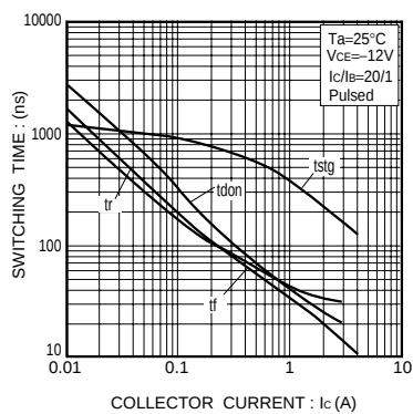
Fig.7 Switching time
