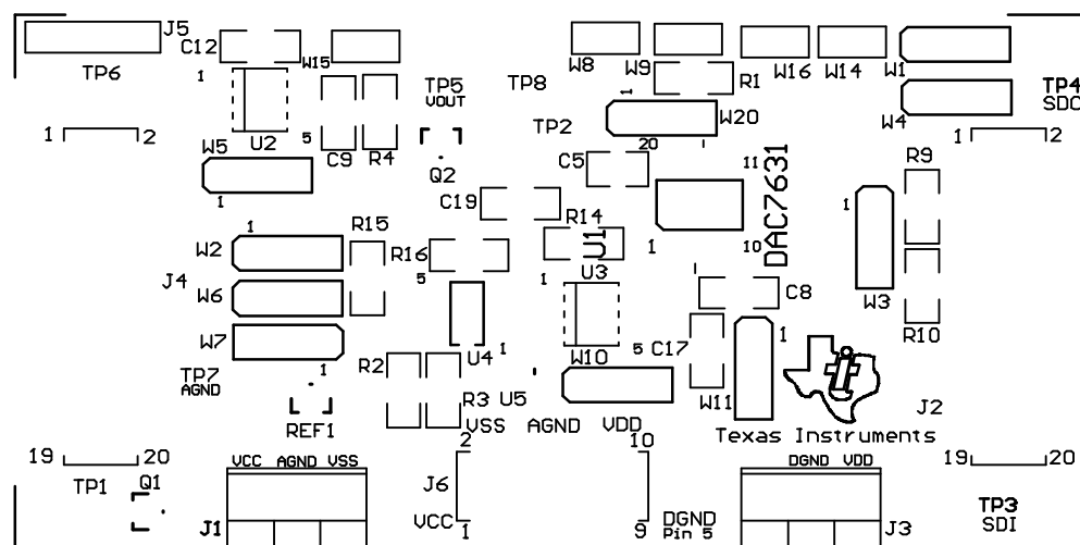
Figure 2. Top Silkscreen
