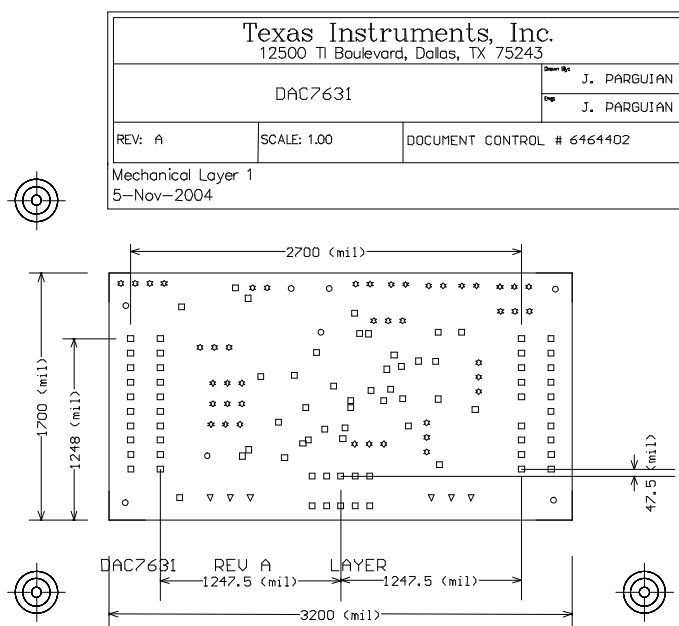
Figure 8. Drill Drawing
