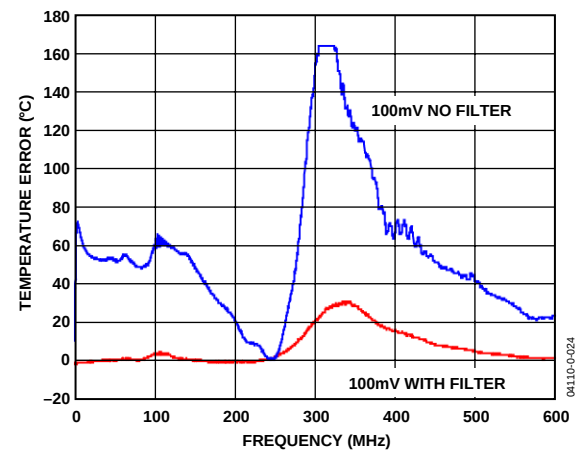
Figure 9. Temperature Error vs. 100 mV Differential Mode Noise Frequency (With and Without R-C-R Filter of 100 \Omega –2.2 nF–100 \Omega )
