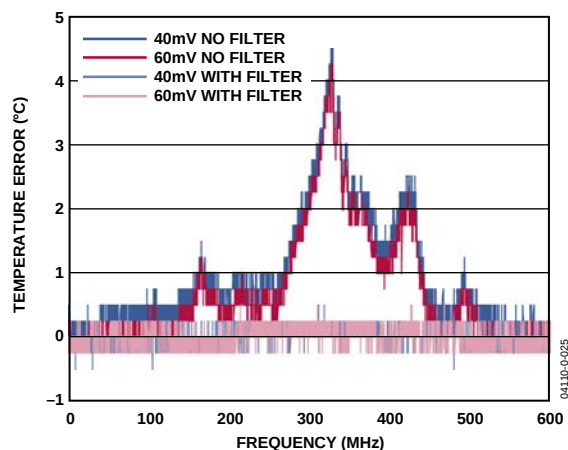
Figure 10. Temperature Error vs. Common-Mode Noise Frequency (With and Without R-C-R Filter of 100 \Omega –2.2 nF–100 \Omega )
