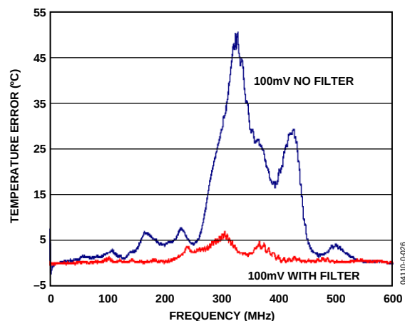
Figure 13. Temperature Error vs. 100 mV Common-Mode Noise Frequency (With and Without R-C-R Filter of 100 \Omega –2.2 nF–100 \Omega )
