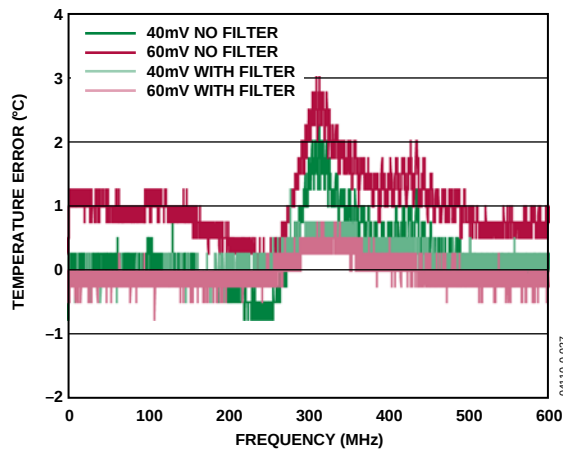
Figure 6. Temperature Error vs. Differential Mode Noise Frequency (With and Without R-C-R Filter of 100 \Omega –2.2 nF–100 \Omega )
