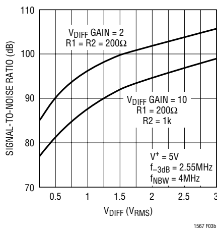
Figure 3. A Single Ended to Differential Amplifier
