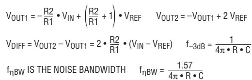
Differential Output Signal-to-Noise Ratio (for a Sinewave Signal)
