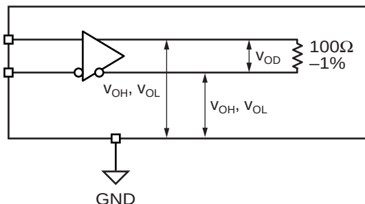
Figure 3a. LVDS Differential Measurement
