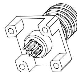
Size 9 PC Board Receptacle
