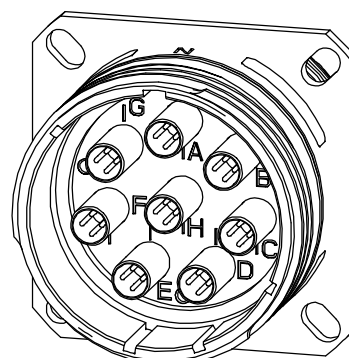
Size 25 Panel Mount Receptacle
