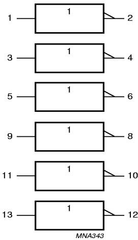
Fig.4 IEC logic symbol.
