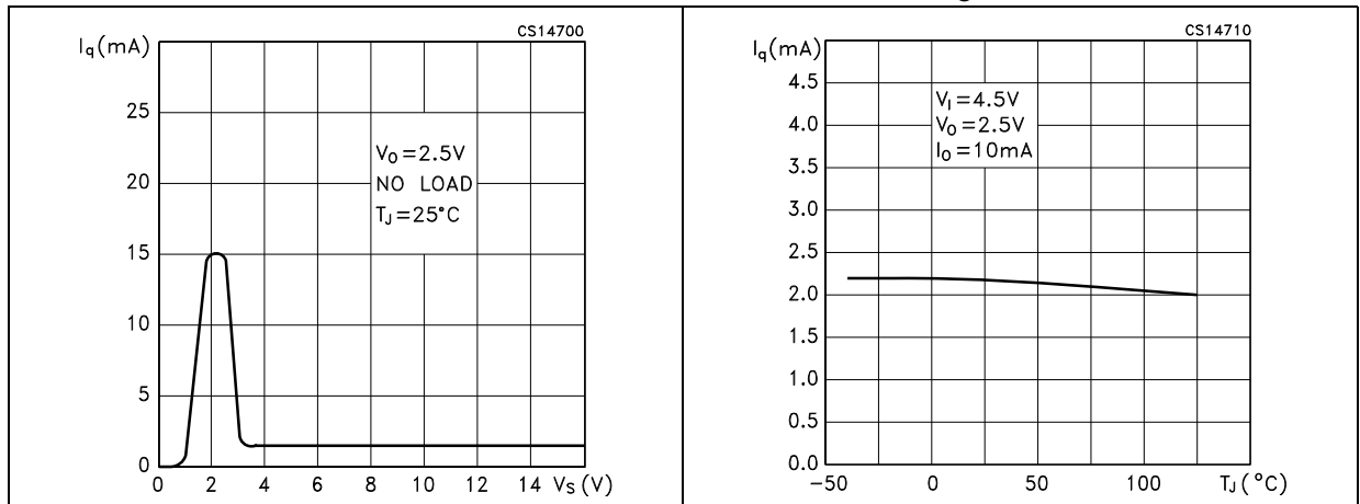
Figure 13. Quiescent current vs. temperature Figure 14. Short circuit current vs. temperature ( I_O = 1.5\text{ A} )
