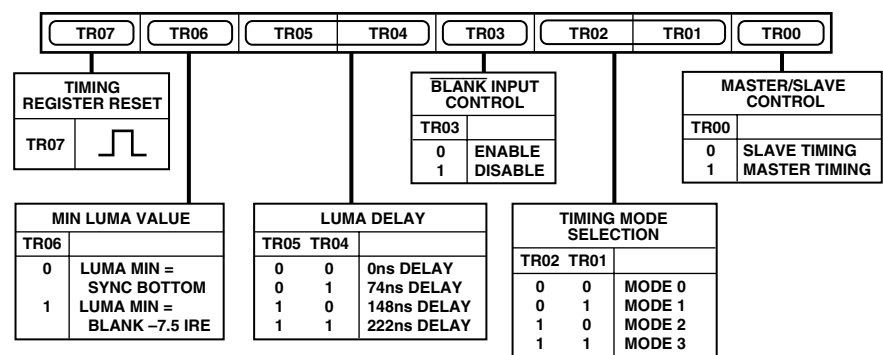
Figure 52. Timing Register 0
