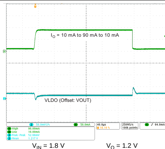
Figure 8-11. Load Transient Response LDO1, LDO2, LDO3
