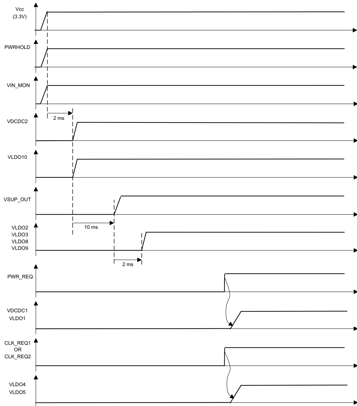
Figure 7-14. TPS659121 3.3-V Host Power Up With CONFIG1=LOW
