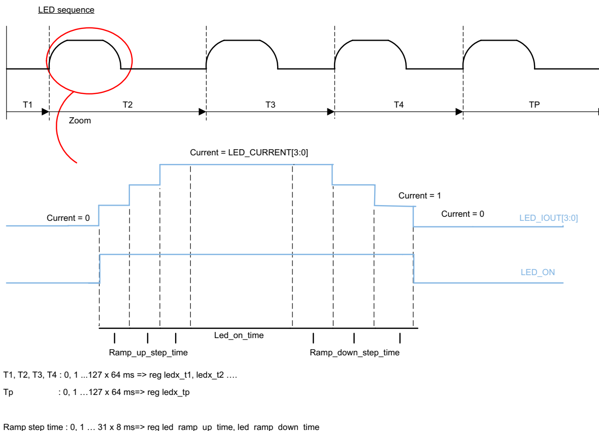
Figure 7-29. LED Sequencer
