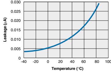
LBA110L Typical Leakage vs. Temperature (Measured across Pins 5 & 6 or 7 & 8)
