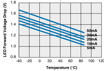
LBA110L Typical LED Forward Voltage Drop vs. Temperature
