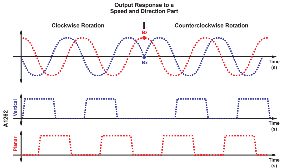
Figure 5: Typical System Timing
