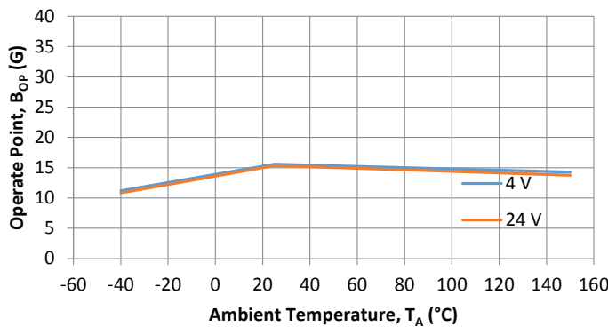
Avg. OUTPUTB Operate Point vs. Ambient Temperature
