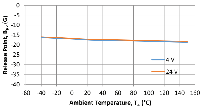
Avg. OUTPUTA Release Point vs. Ambient Temperature
