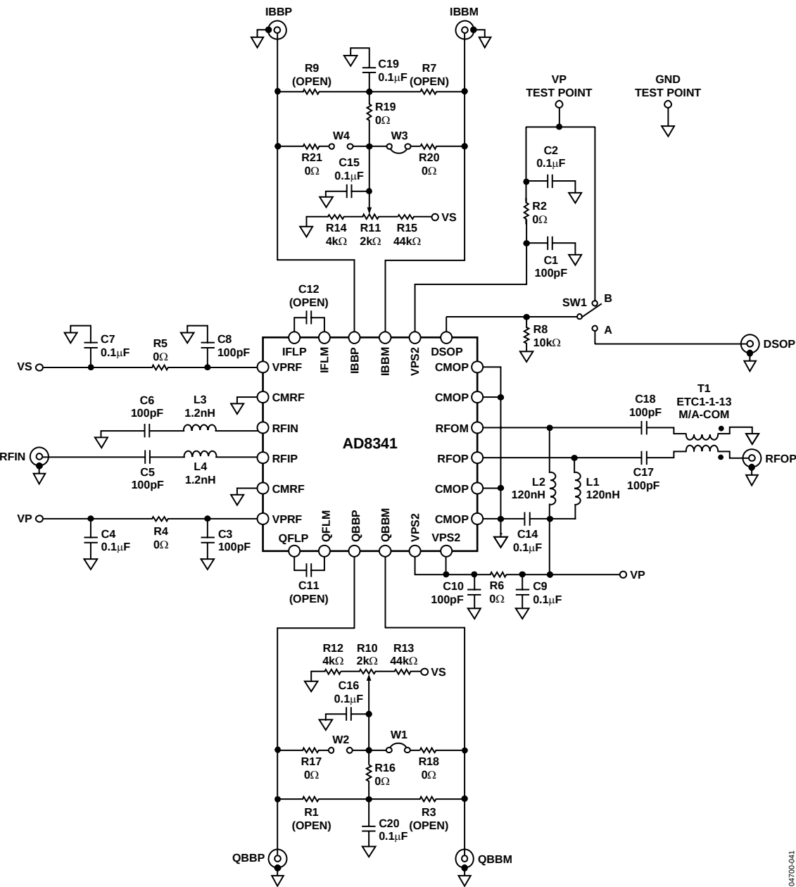
Figure 41. Evaluation Board Schematic
