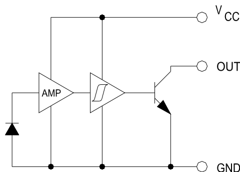
Open-Collector-Output
