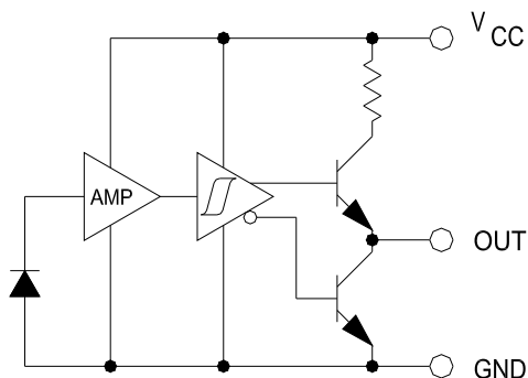
Totem-Pole-Output
