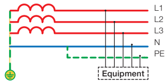
TNC-S system 230/400 V
