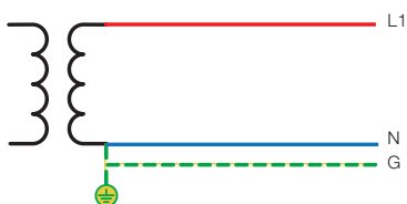
Single phase 120/240/277 V
