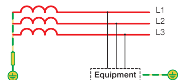
IT system 230/400/600 V
