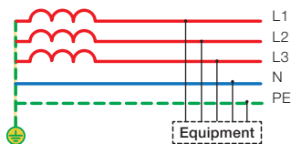
TNS system 230/400 V
