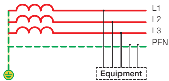
TNC system 230/400 V
