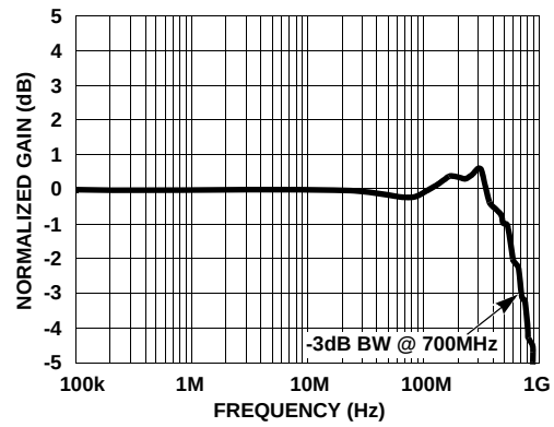
FIGURE 2. -3dB BANDWIDTH
