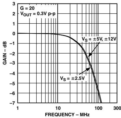
TPC 26. AD8129 Frequency Response vs. Supply, G = 20 , V_{OUT} = 0.3\text{ V p-p}
