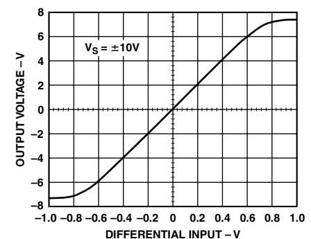
TPC 117. AD8129 Differential Input Clipping Level
