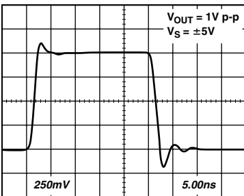
TPC 74. AD8130 Transient Response, V_S = \pm 5\text{ V} , V_{OUT} = 1\text{ V p-p}
