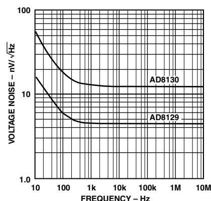
TPC 63. AD8129/AD8130 Input Voltage Noise vs. Frequency
