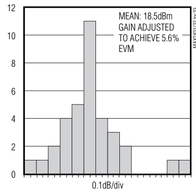
HISTOGRAM: Tx OUTPUT POWER VARIATION
