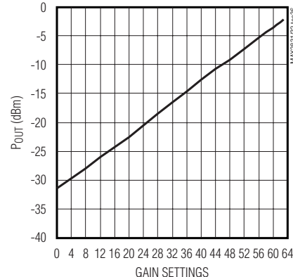
Tx OUTPUT POWER vs. GAIN SETTING (MAX2832 ONLY)
