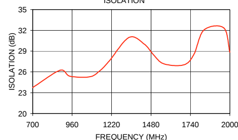
ZAPD-20 ISOLATION
