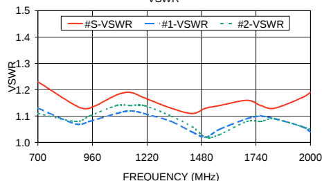
ZAPD-20 VSWR
