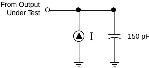
Figure 8. Test Load Diagram
