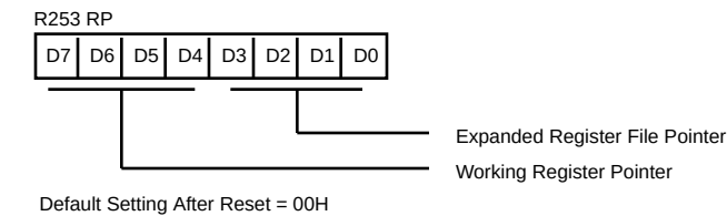
Figure 64. Register Pointer (F DH : Read/Write)
