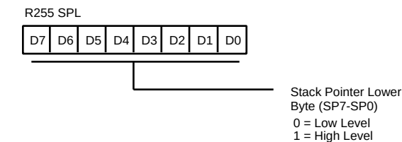
Figure 66. Stack Pointer (F FH : Read/Write)
