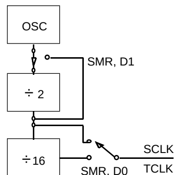
Figure 36. SCLK Circuit
