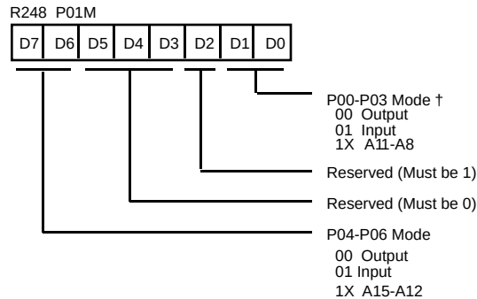
Figure 59. Port 0 and 1 Mode Register (F8 H : Write-Only)
