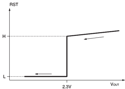
*5 Operation theory for CPU reset circuit
