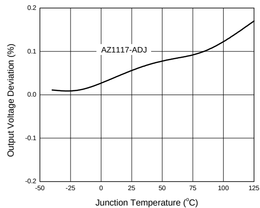
Figure 5. Load Regulation vs. Junction Temperature
