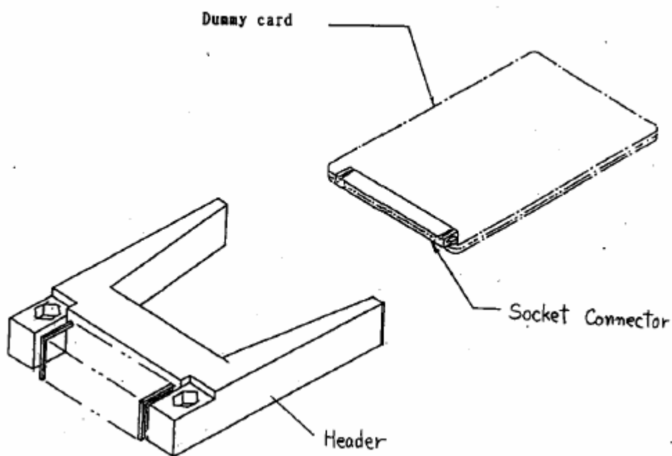
Fig. 5.1 Construction
