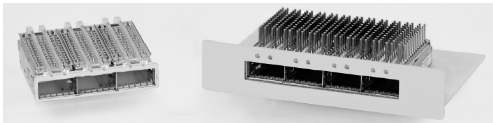
Through Bezel
