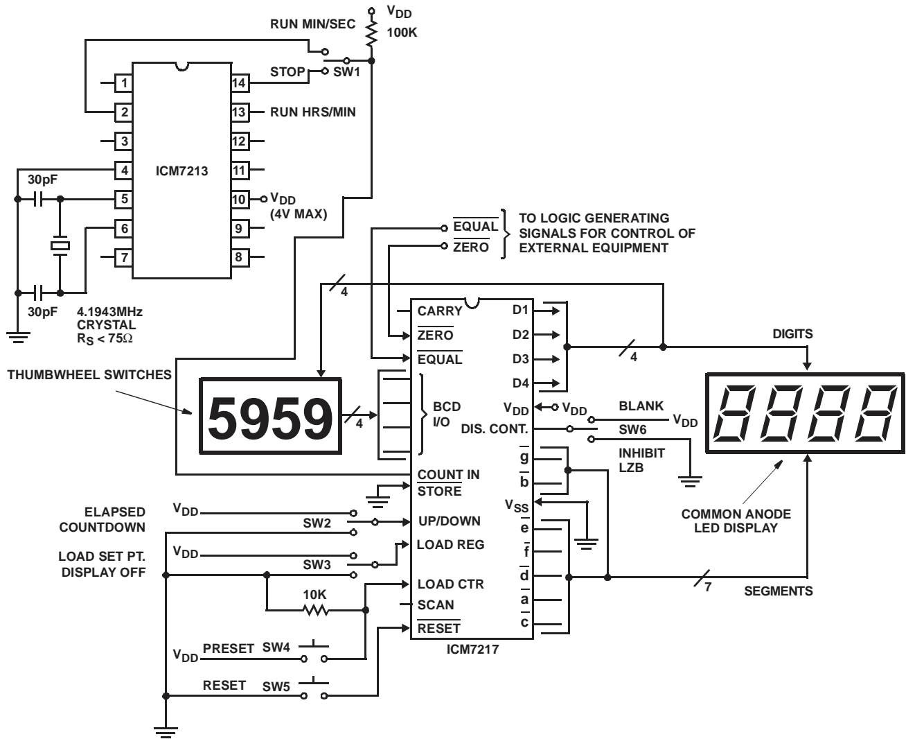
FIGURE 21. PRECISION TIMER
