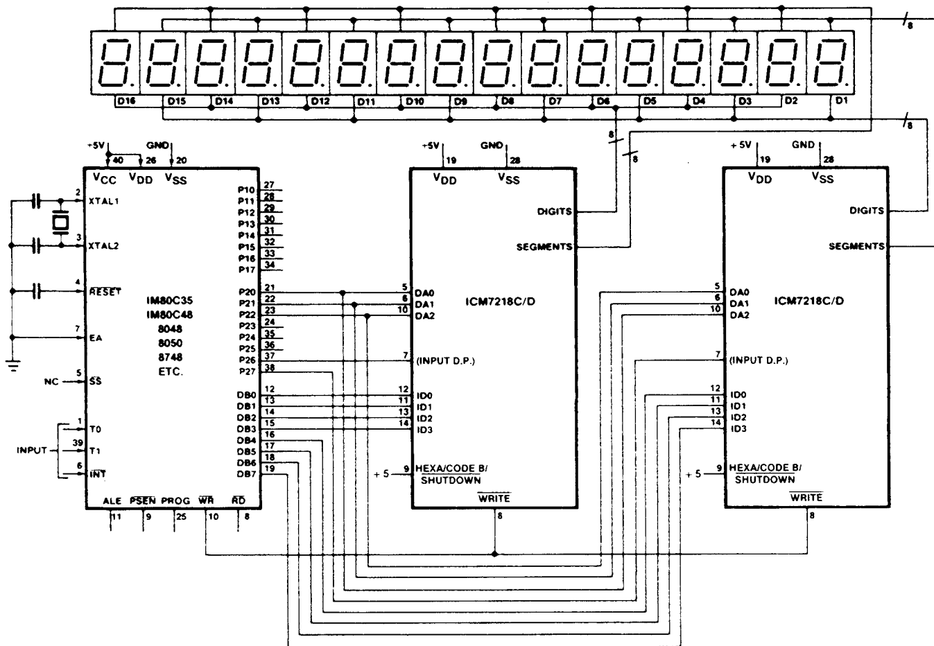
FIGURE 10. 16-DIGIT DISPLAY
