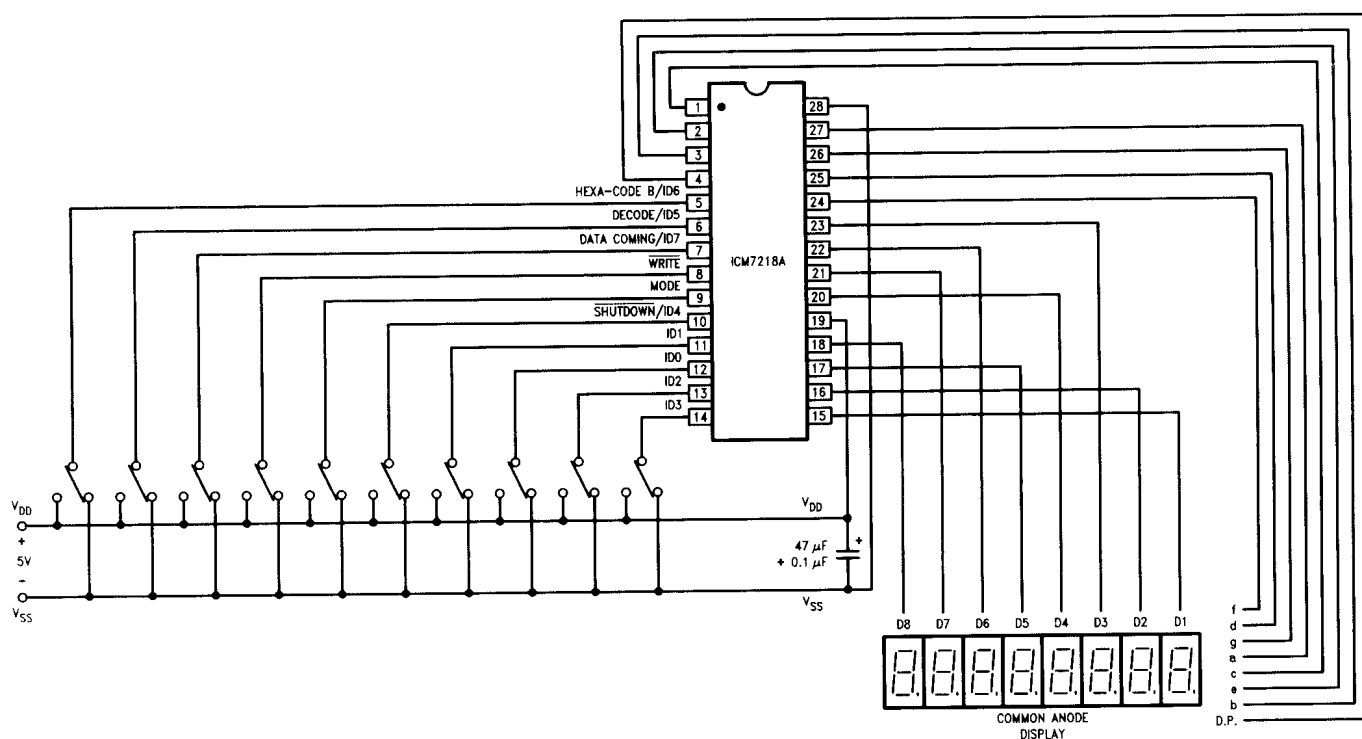
FIGURE 7. COMMON ANODE DISPLAY FUNCTIONAL TEST CIRCUIT
