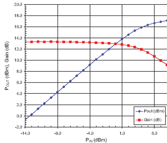
P_{OUT}/Gain versus P_{IN} at 6 GHz
