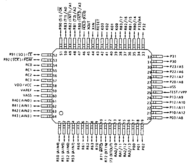
QFP64
