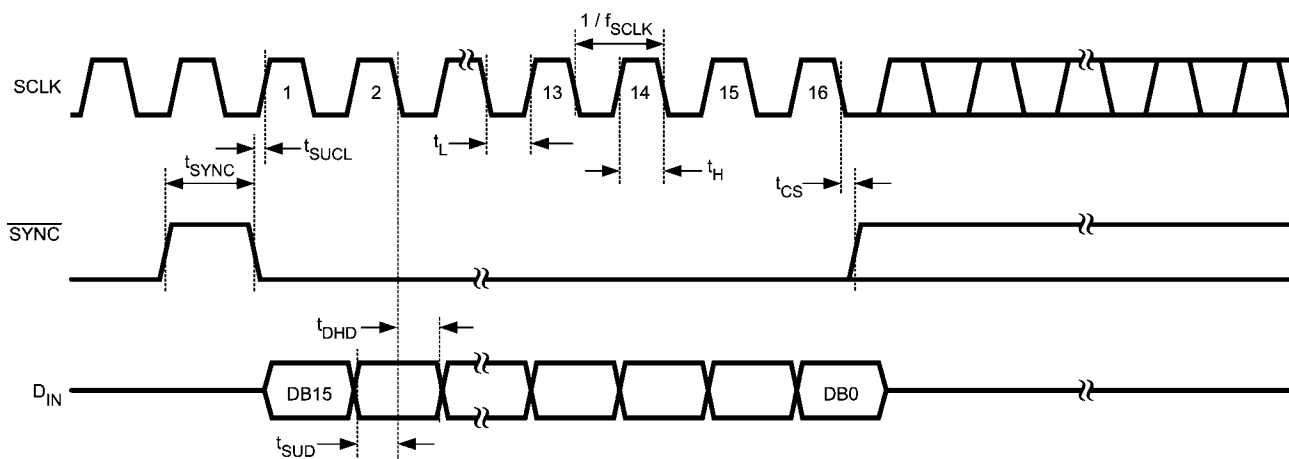
FIGURE 2. DAC121S101 Timing
