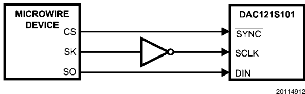
FIGURE 8. Microwire Interface
