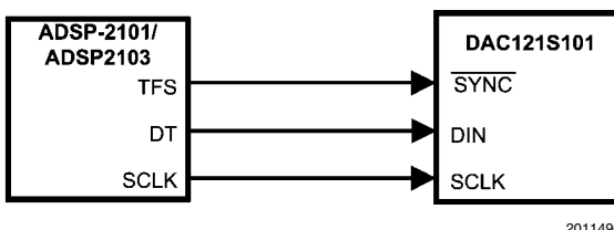
FIGURE 5. ADSP-2101/2103 Interface
