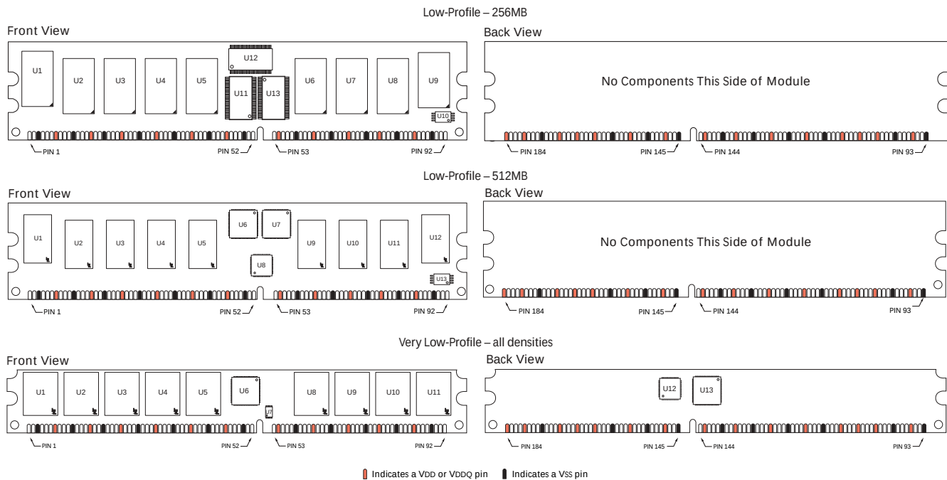
Figure 2: Pin Locations
