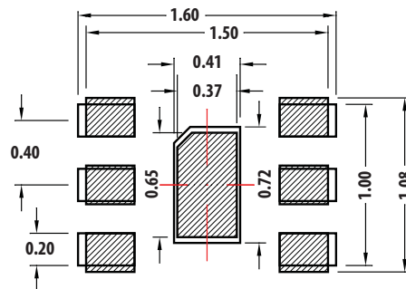
Combination of Land Pattern and Stencil Opening
