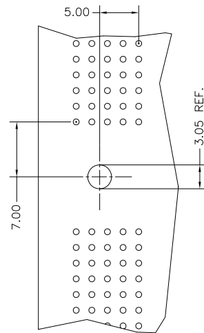
RECOMMENDED HOLE PATTERN WHEN STACKED BESIDE A STANDARD 5 MOD METRAL HEADER COMPONENT SIDE
