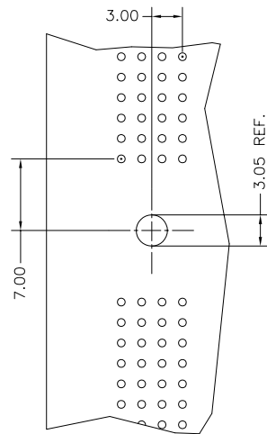
RECOMMENDED HOLE PATTERN WHEN STACKED BESIDE A STANDARD 4 MOD METRAL HEADER COMPONENT SIDE
