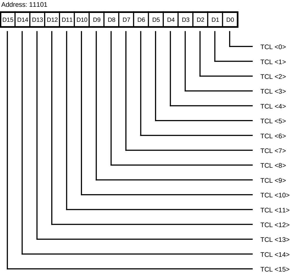
Figure 76. Transmit Count Limit Register (TCLR)
