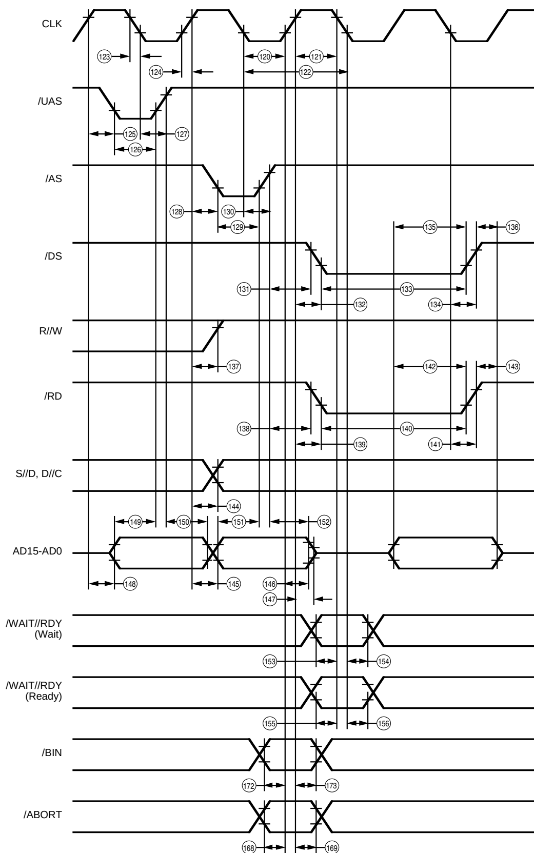
Figure 102. Memory Read
