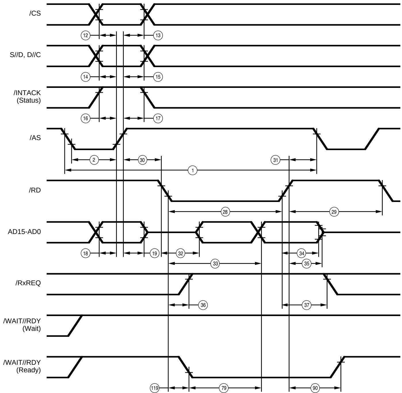
Figure 87. Multiplexed \overline{\text{RD}} Read Cycle
