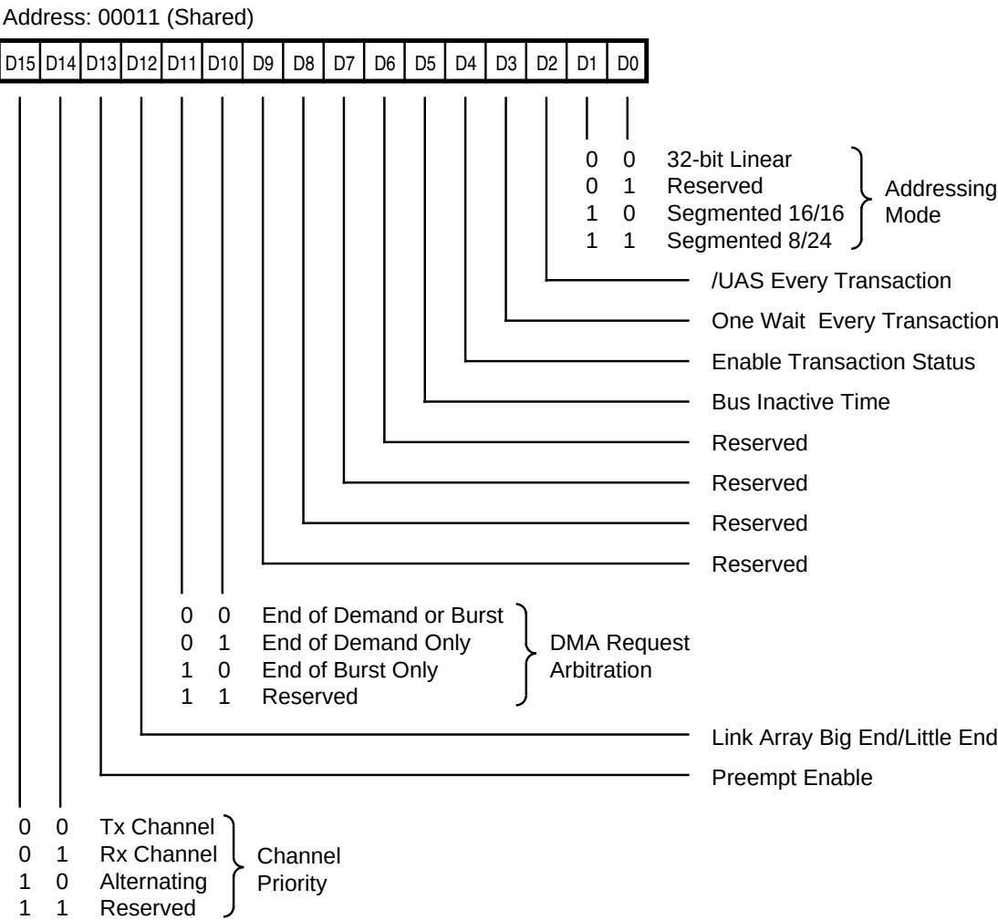
Figure 12. DMA Control Register (DCR)
