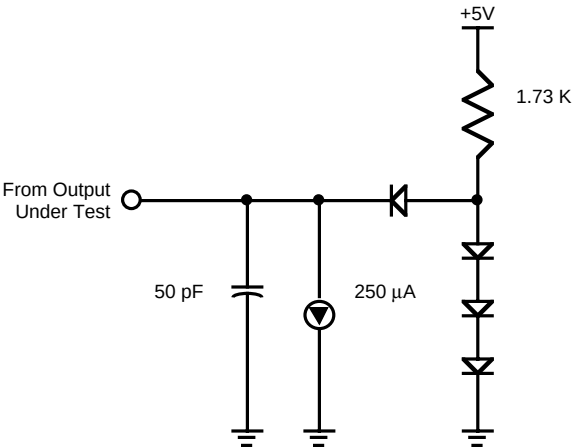
Figure 82. Standard Test Load
